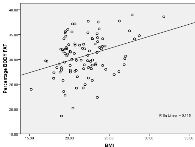
Figure 1: Scatter plot showing distribution of PBF with respect to BMI (overall)
