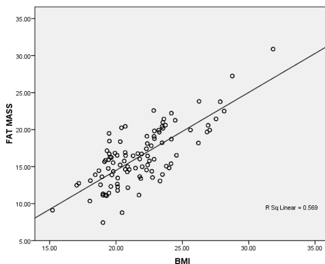
Figure 2; Relationship between BMI and Fat Mass
